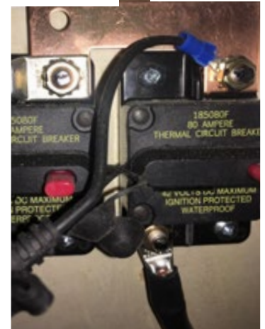
80 AMP BATTERY DISCONNECT BREAKER 80 AMP GENERATOR BREAKER
