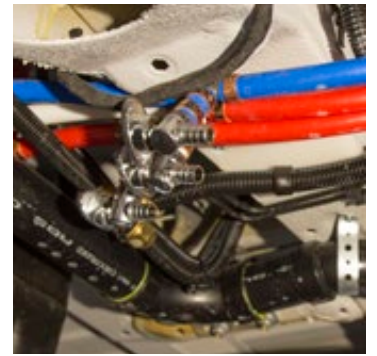
RED: Hot water line BLUE: Cold water line WHITE: Recirculation line
