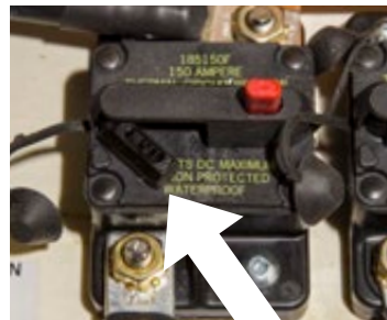
ARM DOWN INDICATES TRIPPED BREAKER
